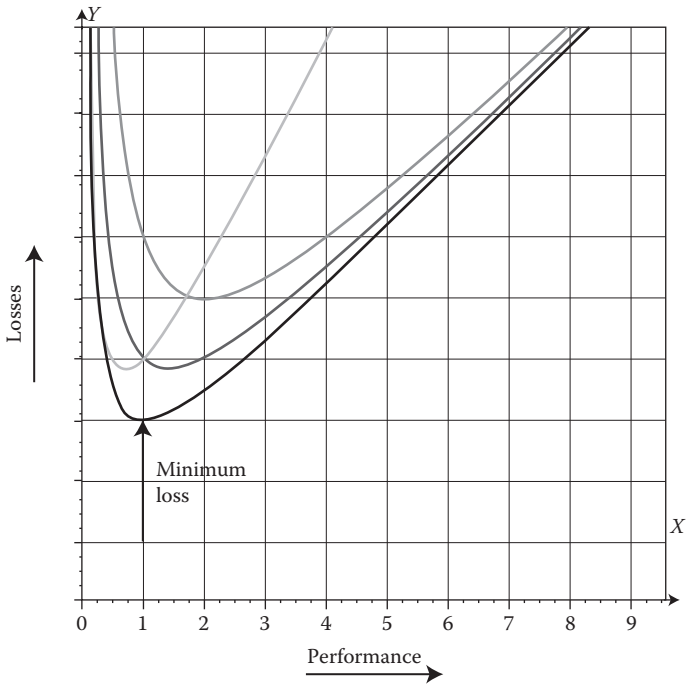
FIGURE A2.4 Pareto-efficient quality loss function optimized for minimum loss.
