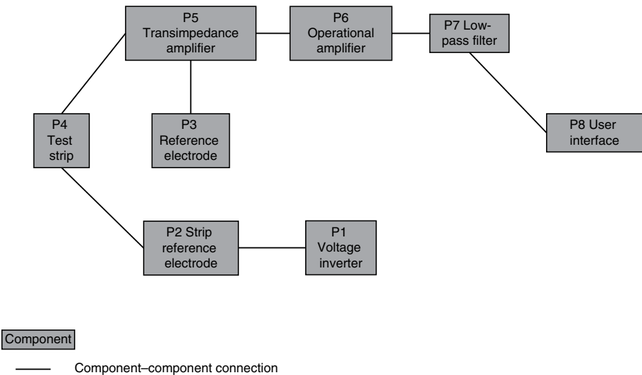
Figure 9.2. Glucose meter example physical architecture.
