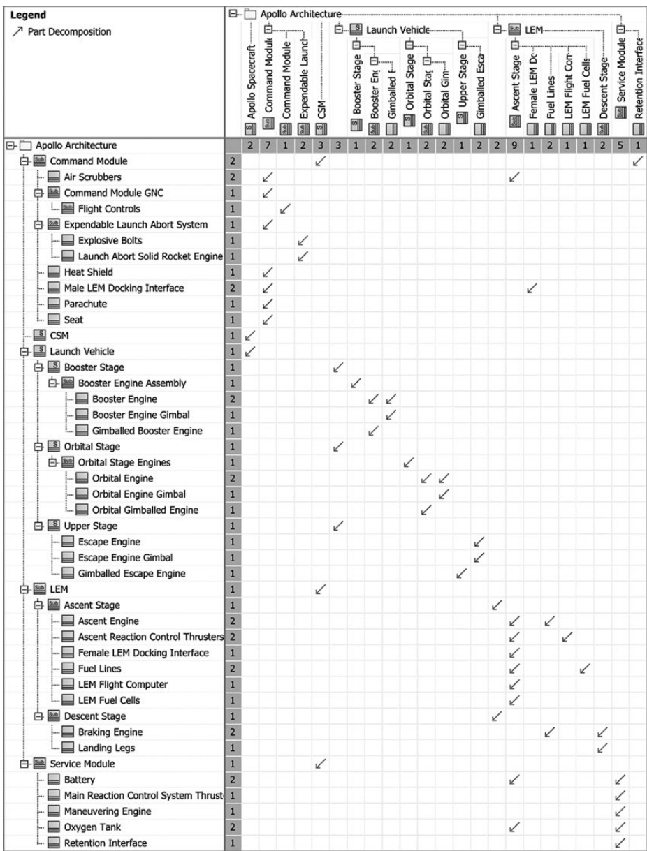
Figure 10.3. Apollo part decomposition matrix.
