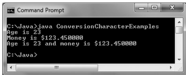
Figure C-7 Output of the ConversionCharacterExamples application
