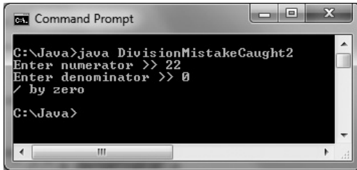
Figure 12-10 Output of the DivisionMistakeCaught2 application
