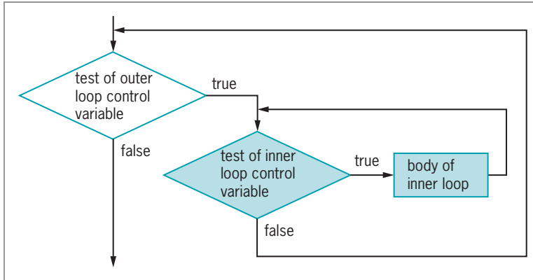
Figure 6-23 Nested loops
