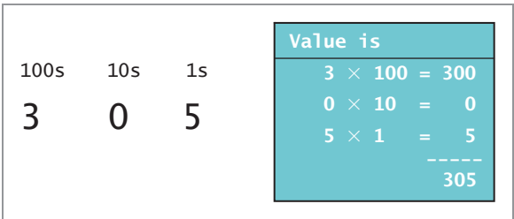
Figure B-1 Representing 305 in the decimal system
