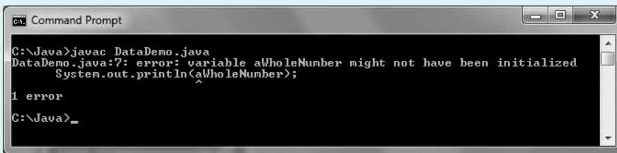
Figure 2-7 Error message generated when a variable is not initialized
