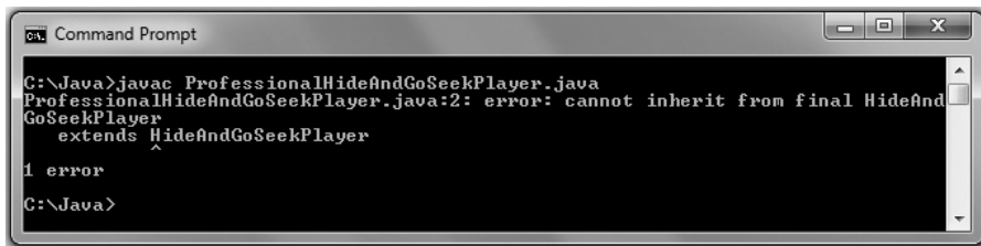
Figure 10-29 Error message when compiling the ProfessionalHideAndGoSeekPlayer class in Figure 10-28
