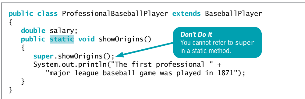
Figure 10-20 The ProfessionalBaseballPlayer class with a static method that attempts to reference super
