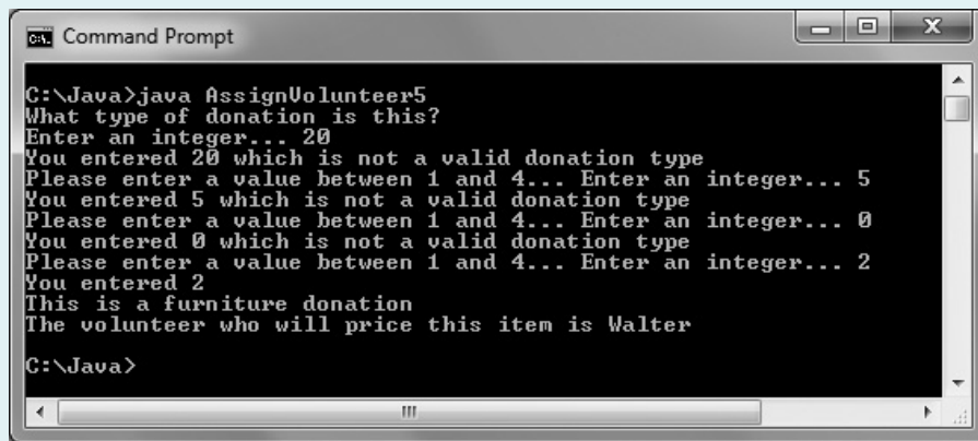
Figure 6-12 Typical execution of the AssignVolunteer5 application
