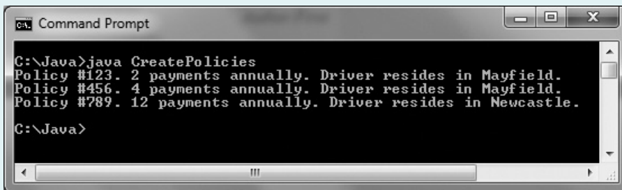
Figure 4-23 Output of the CreatePolicies program
