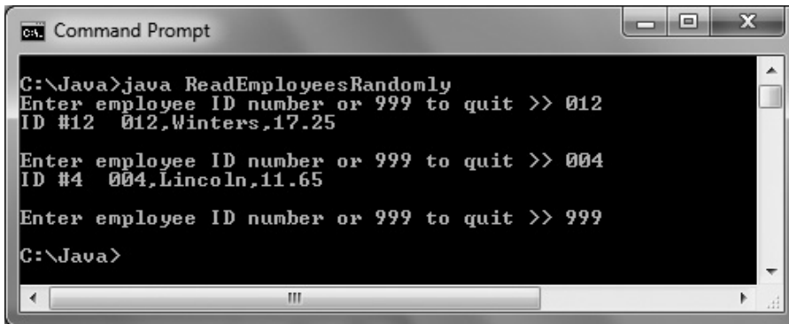
Figure 13-40 Typical execution of the ReadEmployeesRandomly program
