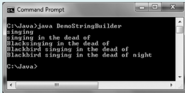
Figure 7-19 Output of the DemoStringBuilder application
