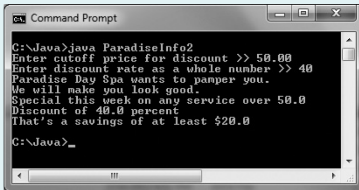
Figure 3-22 Typical execution of the ParadiseInfo2 program
