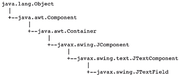
Figure 14-19 The JTextField class inheritance hierarchy
