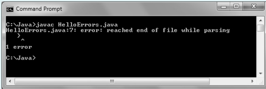
Figure 1-16 Error message generated when the closing curly brace is omitted from the HelloErrors program
