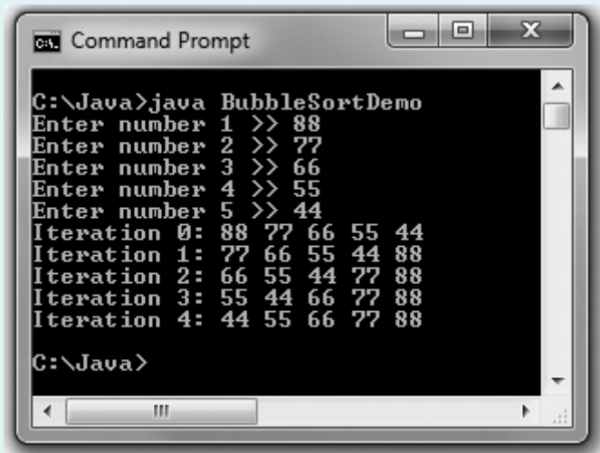
Figure 9-5 Typical execution of the BubbleSortDemo application
