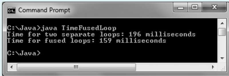
Figure 6-31 Execution of the TimeFusedLoop program
