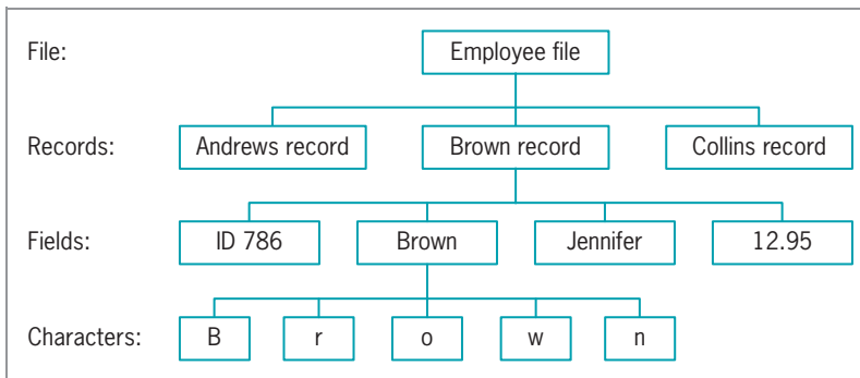
Figure 13-12 Data hierarchy
