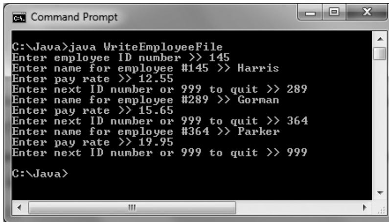
Figure 13-22 Typical execution of the WriteEmployeeFile program
