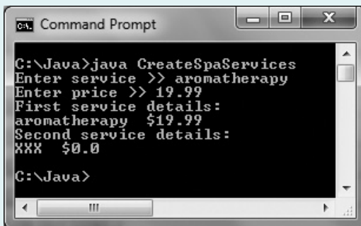
Figure 3-33 Typical execution of CreateSpaServices program that uses constructor values for the second object
