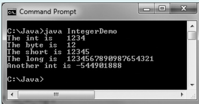
Figure 2-13 Output of the modified IntegerDemo program with an out-of-range integer
