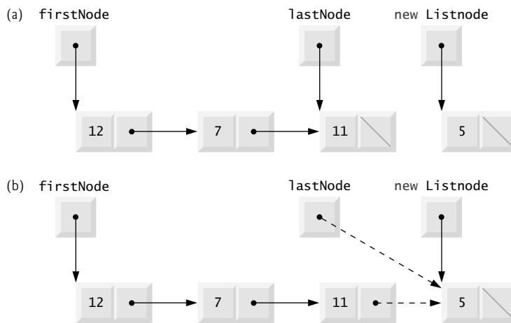
Fig. 21.7 | Graphical representation of operation insertAtBack .
