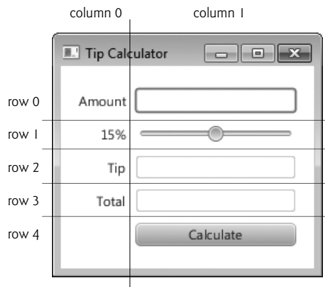
Fig. 25.10 | Tip Calculator GUI's GridPane labeled by its rows and columns.
