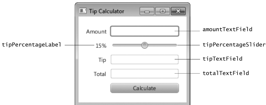
Fig. 25.11 | Tip Calculator's programmatically manipulated controls labeled with their fx:ids .
