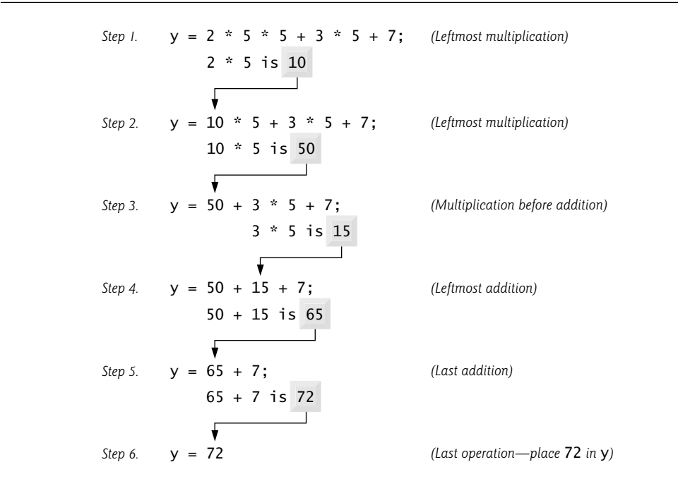
Fig. 2.13 | Order in which a second-degree polynomial is evaluated.
