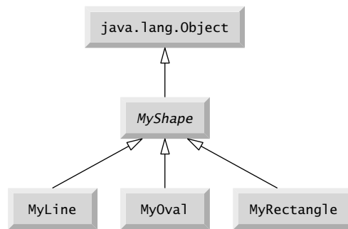
Fig. 10.17 | MyShape hierarchy.
