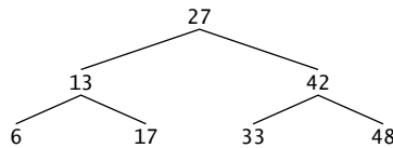
Fig. 21.19 | Binary search tree with seven values.
