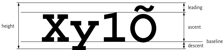
Fig. 13.13 | Font metrics.
