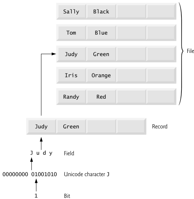
Fig. I.3 | Data hierarchy.
