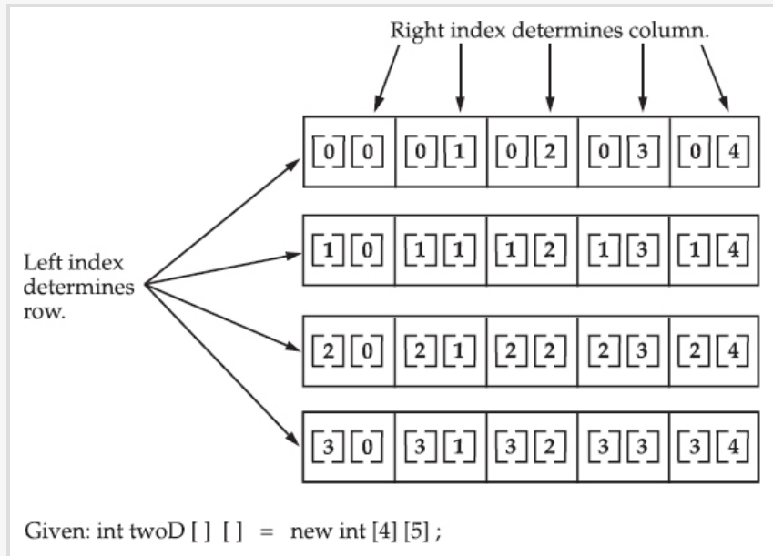
Figure 3-1 A conceptual view of a 4 by 5, two-dimensional array
