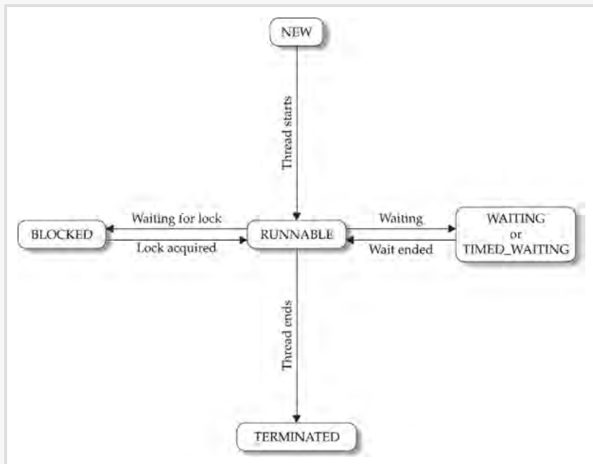
Figure 11-1 diagrams how the various thread states relate.
