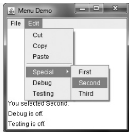
Figure 26-8 Sample output from the MenuDemo applet
