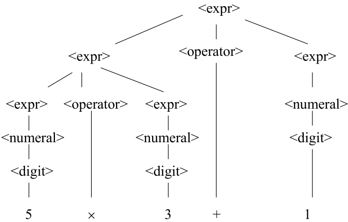
Fig. 12.2 Parse tree 5 × 3 + 1 (multiplication first)
