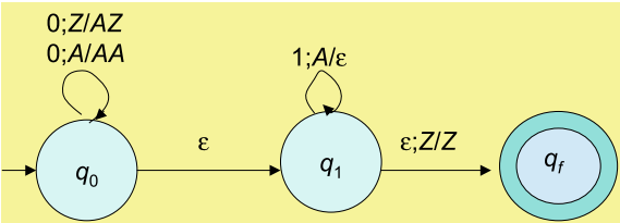
Fig. 7.6 Transition function for pushdown automata M
