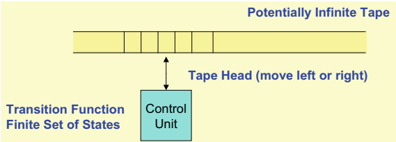
Fig. 7.7 Turing machine
