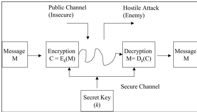
Fig. 10.6 Symmetric key cryptosystem
