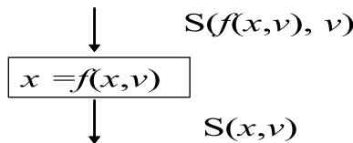
Fig. 18.7 Assignment assertions in flowcharts
