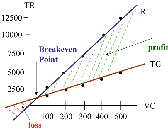
Fig. 24.4 Breakeven point
