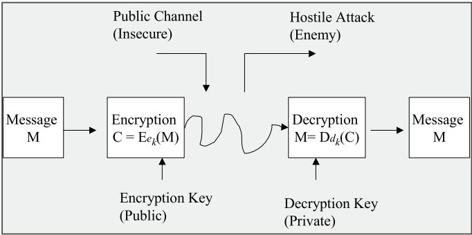
Fig. 10.7 Public key cryptosystem
