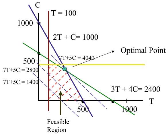
Fig. 24.3 Optimal solution
