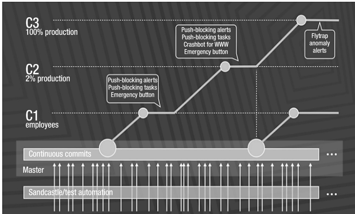
Figure 1-10 Rapid release at massive scale. Source: Rossi, Chuck; “Rapid Release at Massive Scale,” August 31, 2017, https://code.facebook.com/posts/270314900139291/rapid-release-at-massive-scale/
