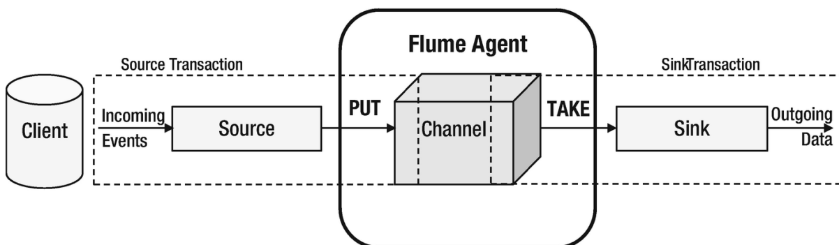
Figure 2-17 Apache Flume architecture
