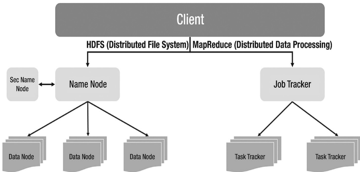
Figure 6-5 Hadoop storage and processing framework
