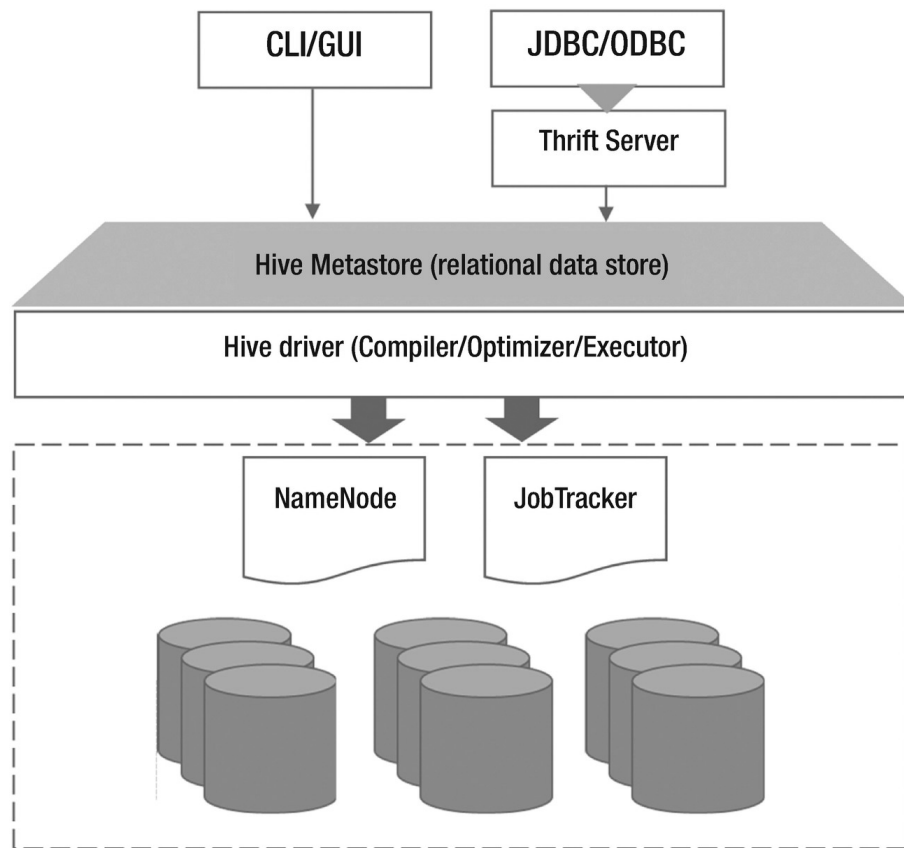
Figure 4-6 Hive architecture
