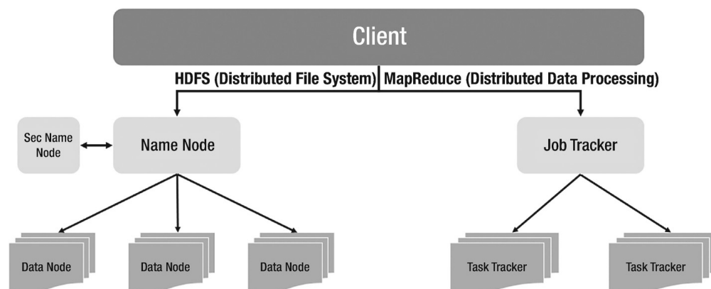
Figure 4-1 A classical MapReduce operation
