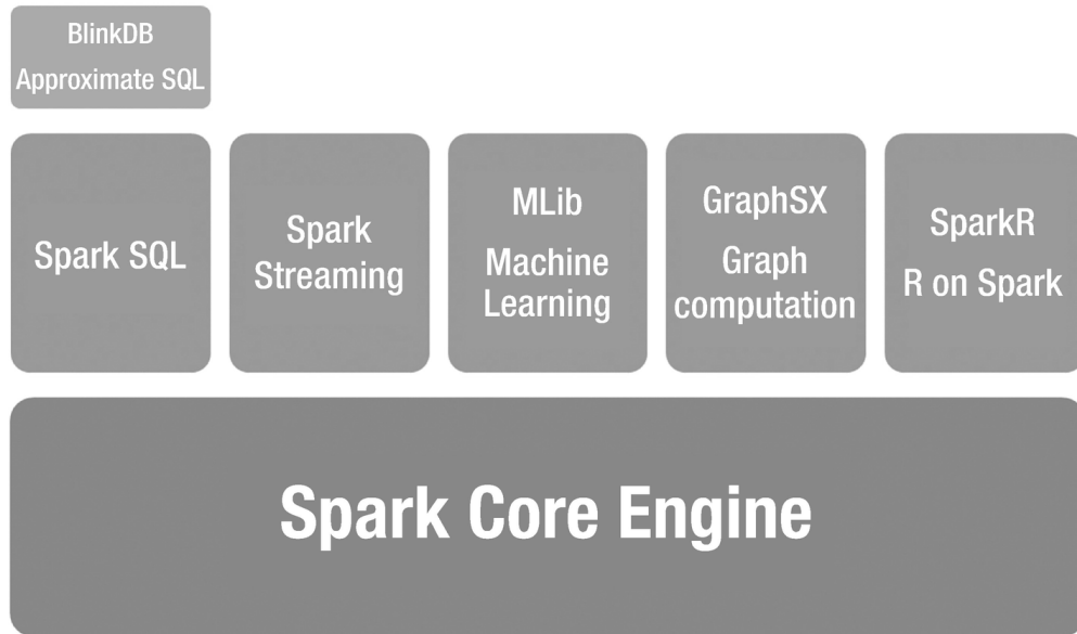
Figure 4-12 Spark Stack
