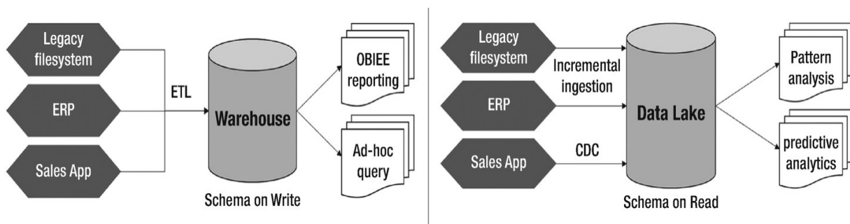
Figure 1-9 Data warehouse versus Data Lake
