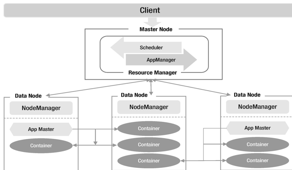
Figure 4-4 Subcomponent level design of YARN
