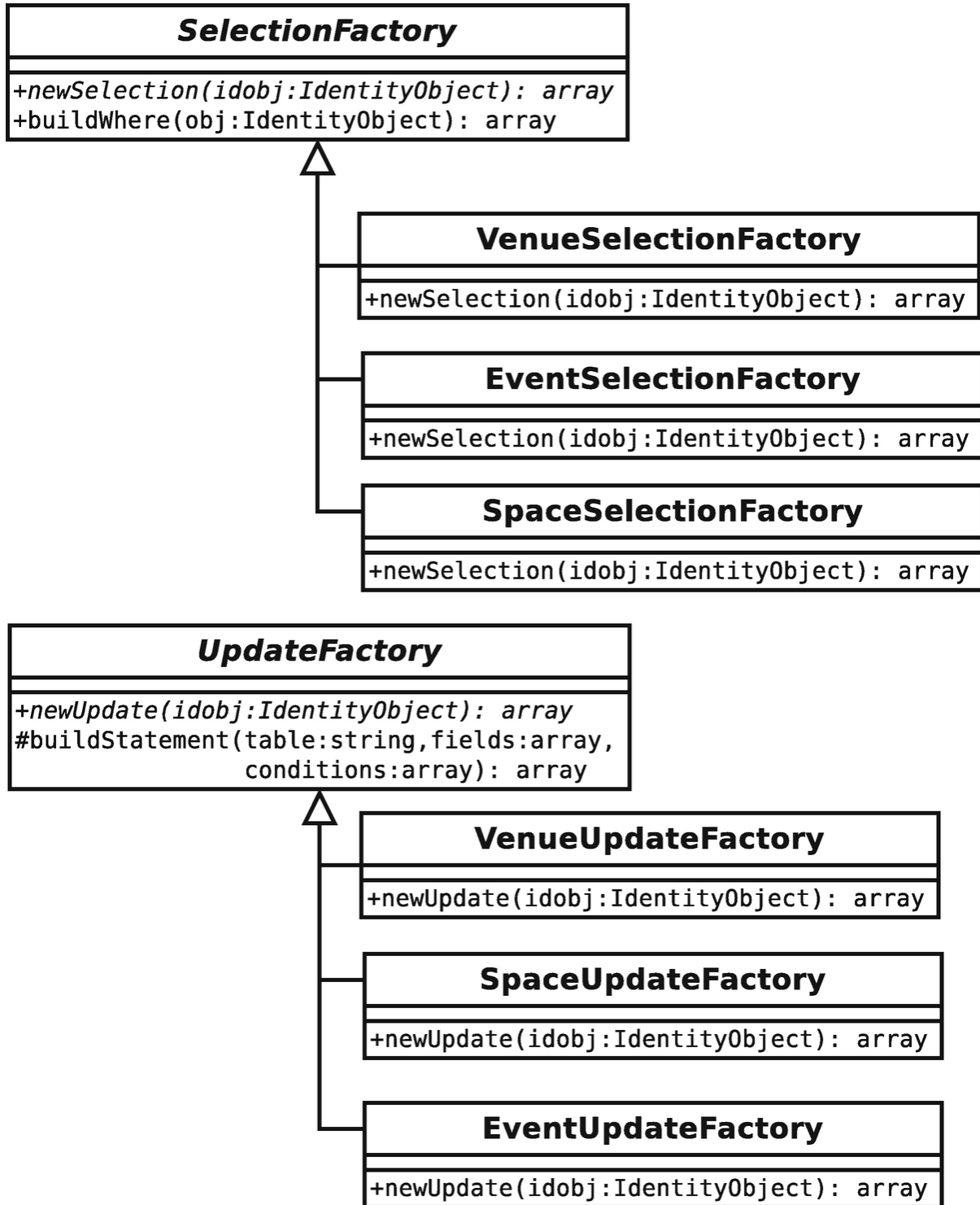
Figure 13-9 Selection and update factories
