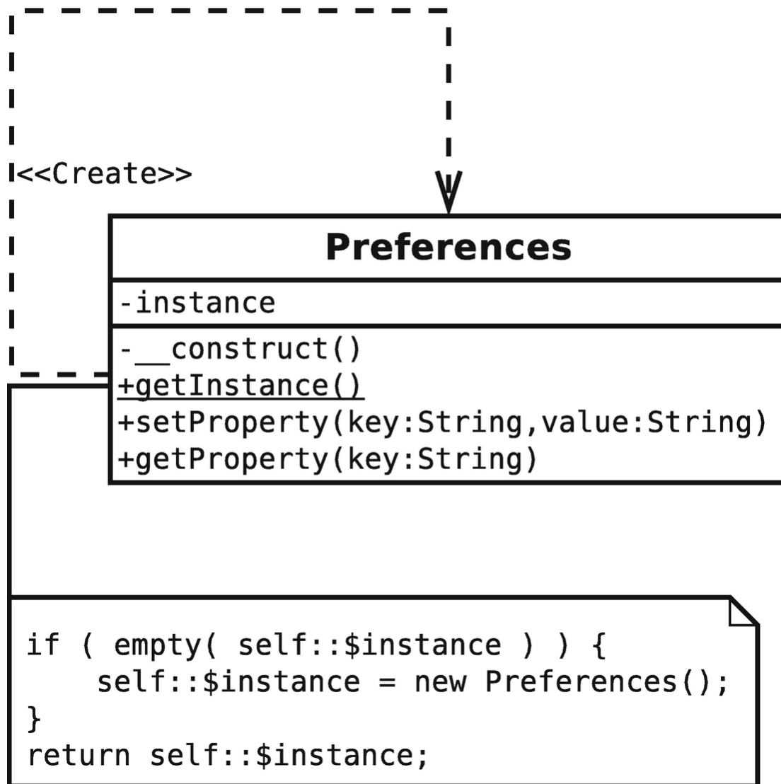
Figure 9-2 An example of the Singleton pattern
