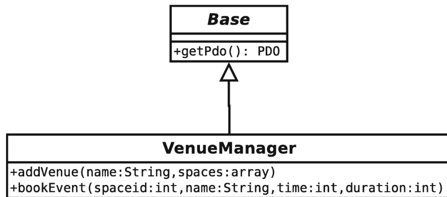
Figure 12-10 A Transaction Script class with its superclass
