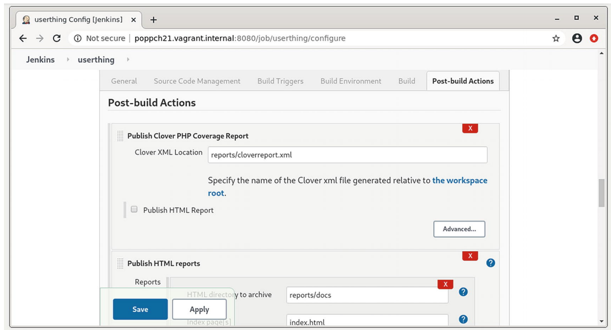
Figure 21-10 Configuring report plug-in items
