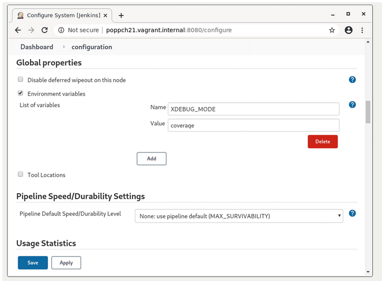
Figure 21-11 Setting an environment variable
