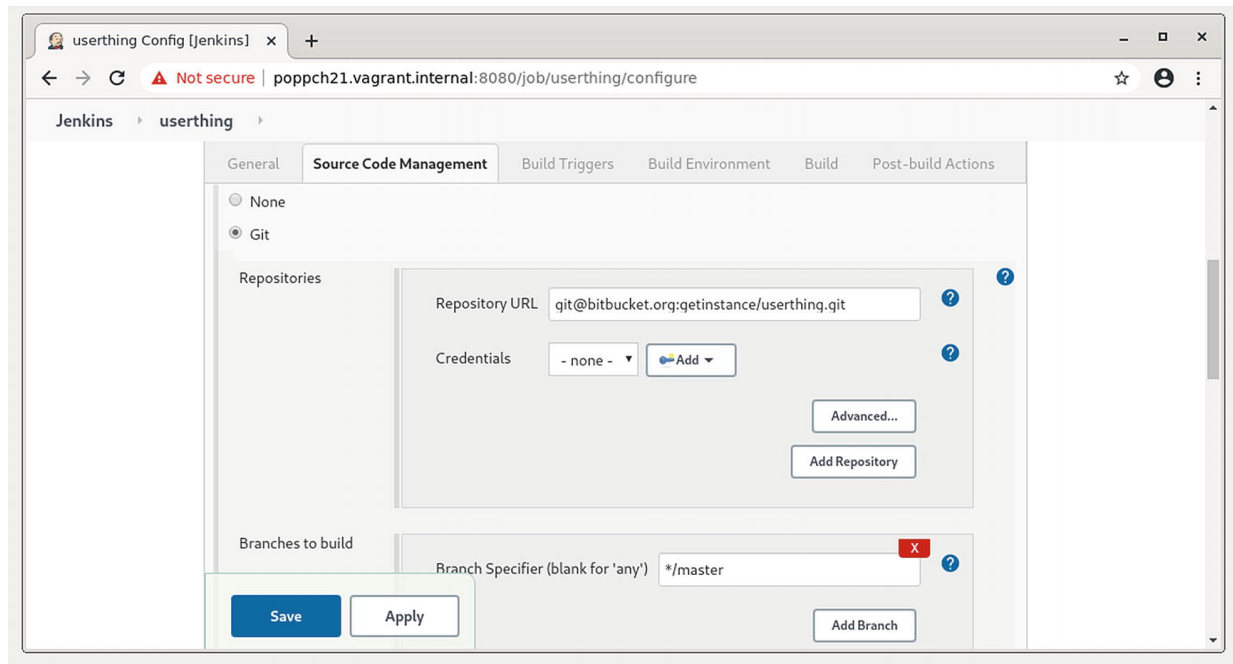
Figure 21-5 Setting up the version control repository
