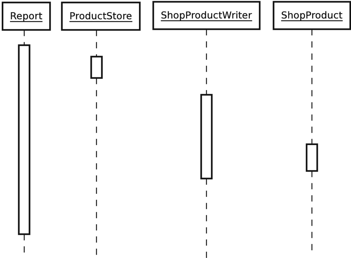
Figure 6-19 Object lifelines in a sequence diagram
