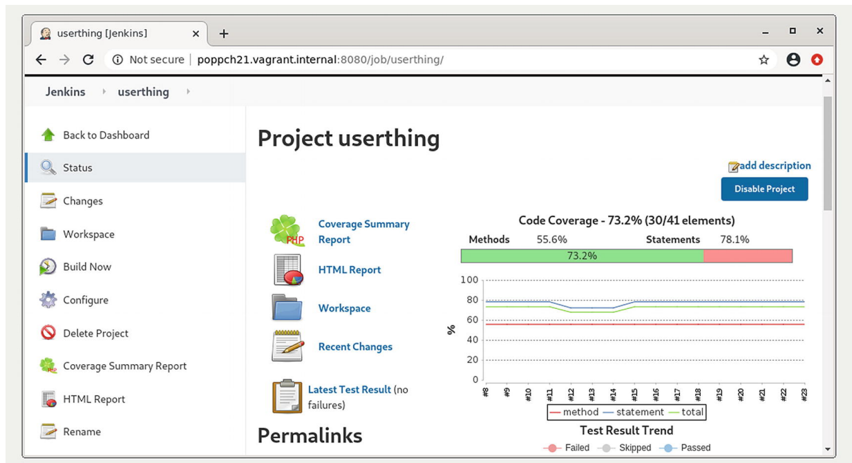
Figure 21-12 The project screen showing trend information
