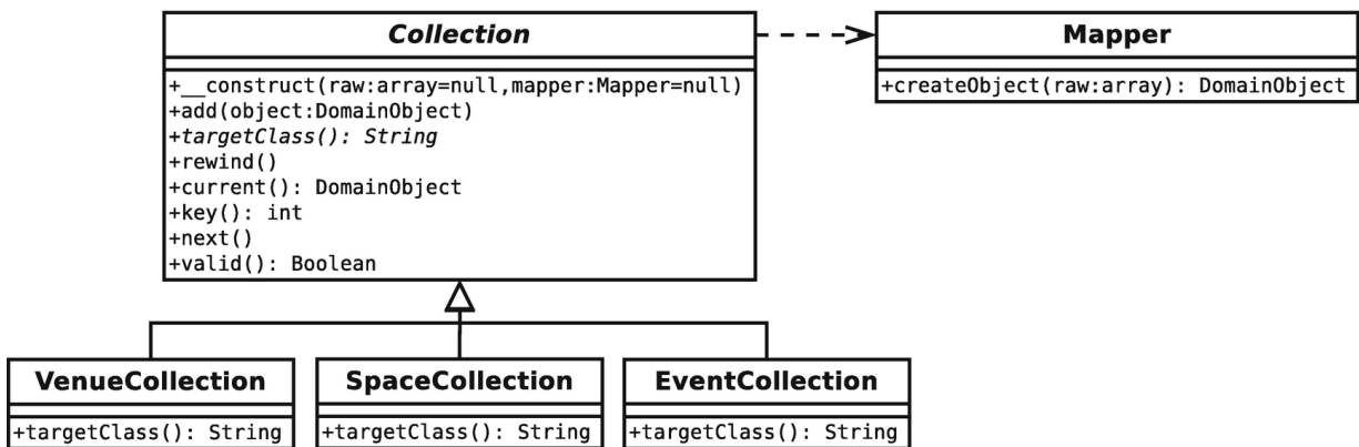
Figure 13-2 Managing multiple rows with collections
