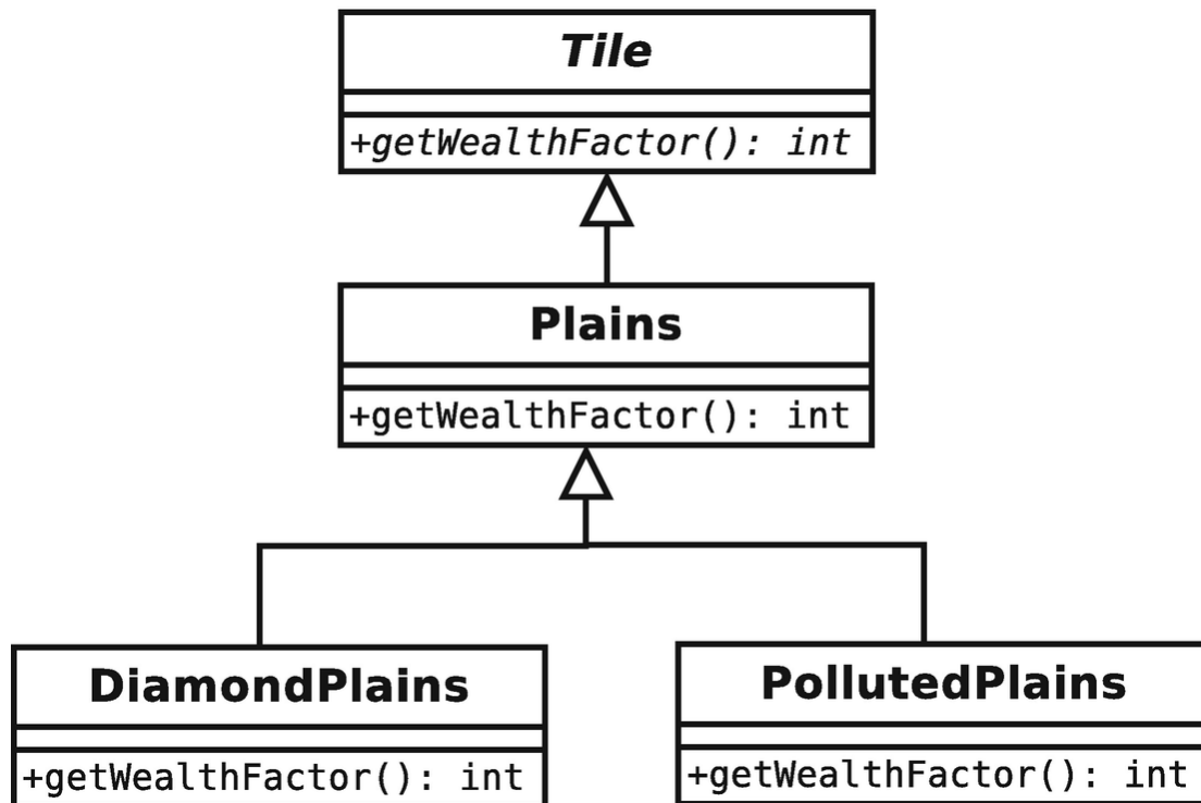
Figure 10-3 Building variation into an inheritance tree
