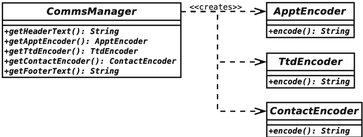
Figure 9-7 An abstract creator and its abstract products
