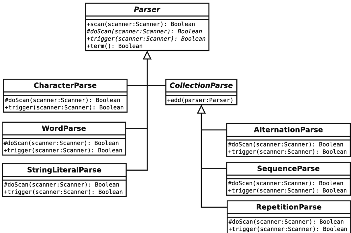
Figure B-1 The Parser classes
