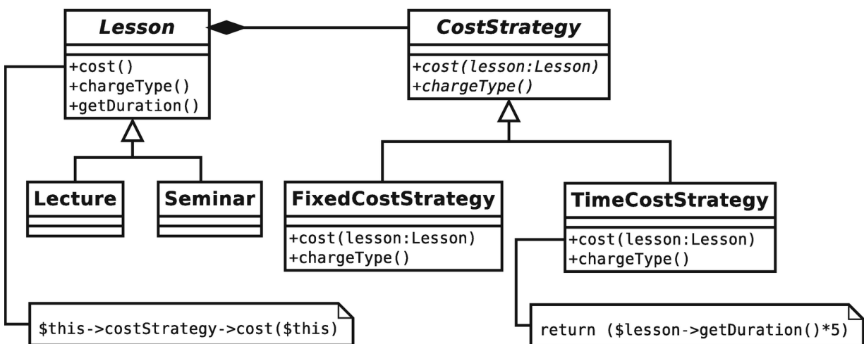
Figure 8-4 Moving algorithms into a separate type
