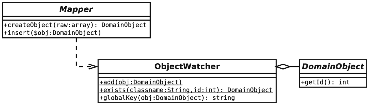
Figure 13-4 An Identity Map
