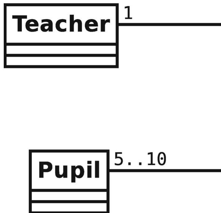
Figure 6-13 Defining multiplicity for an association
