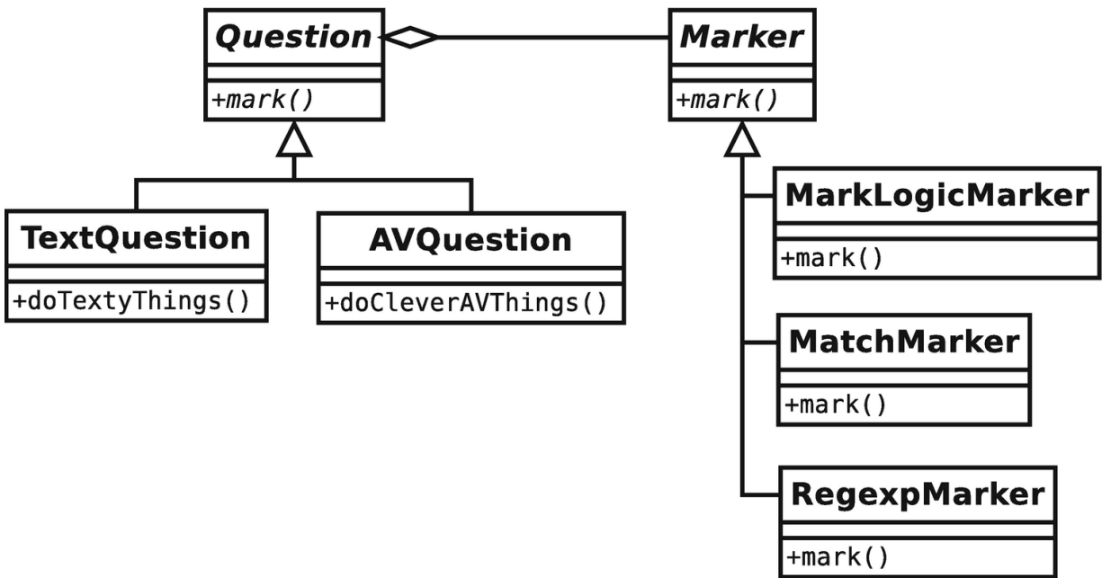
Figure 11-5 Extracting algorithms into their own type
