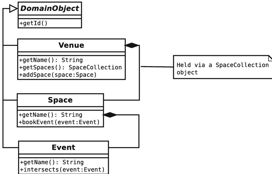
Figure 12-11 An extract from a Domain Model
