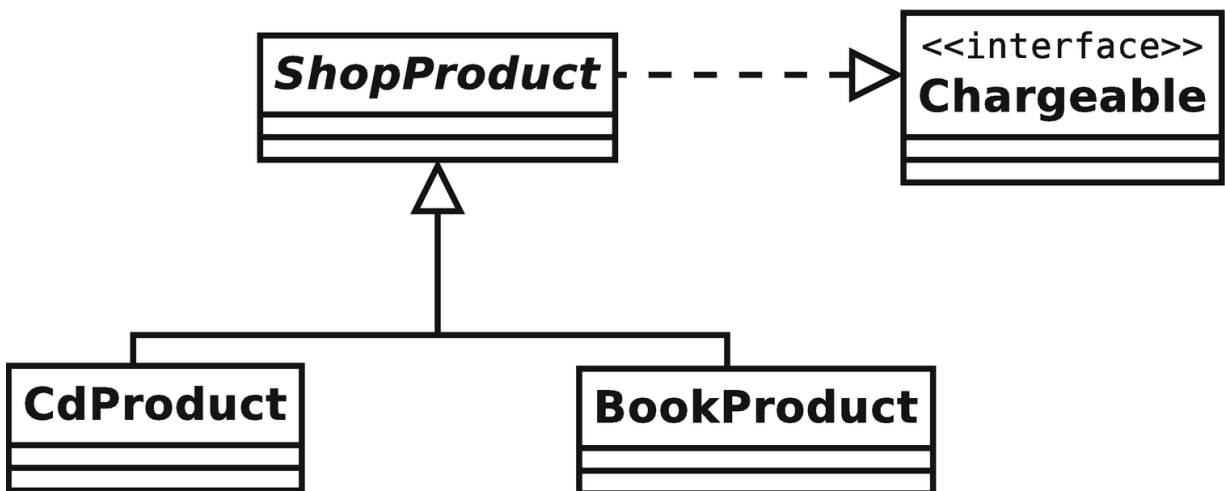
Figure 6-8 Describing interface implementation
