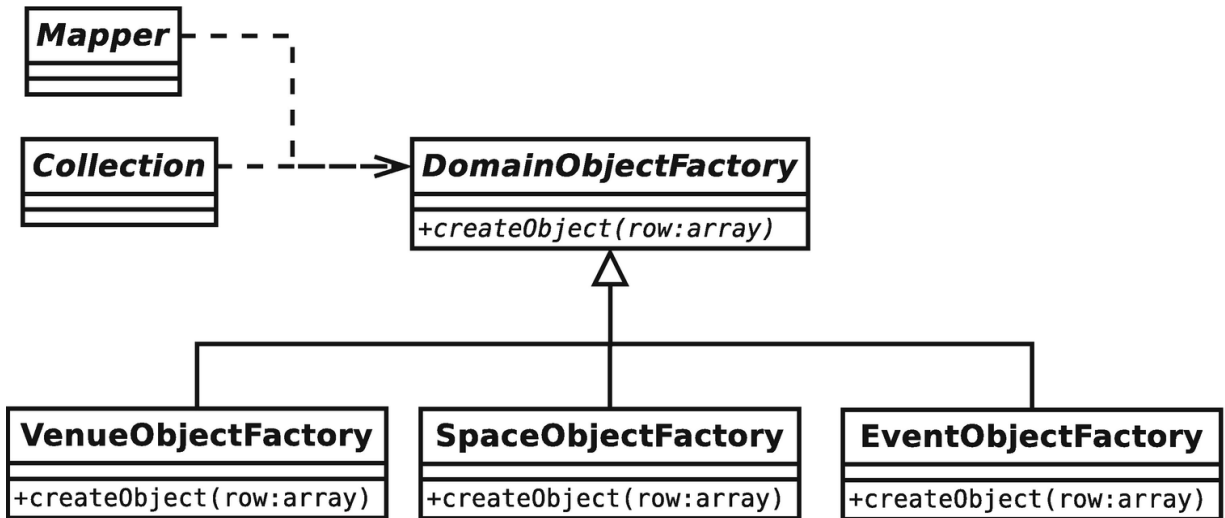
Figure 13-6 Domain Object Factory classes
