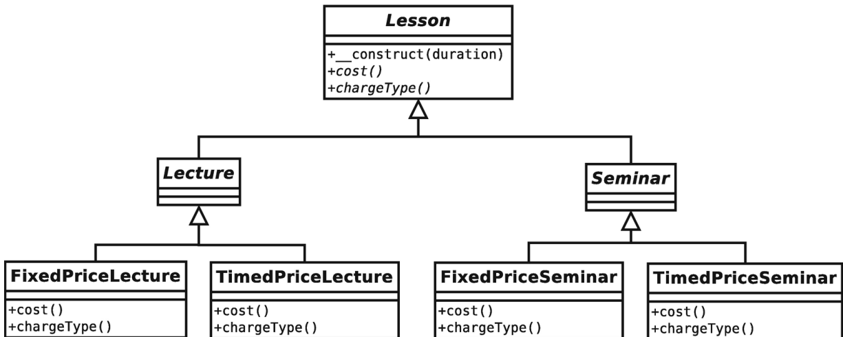
Figure 8-2 A poor inheritance structure
