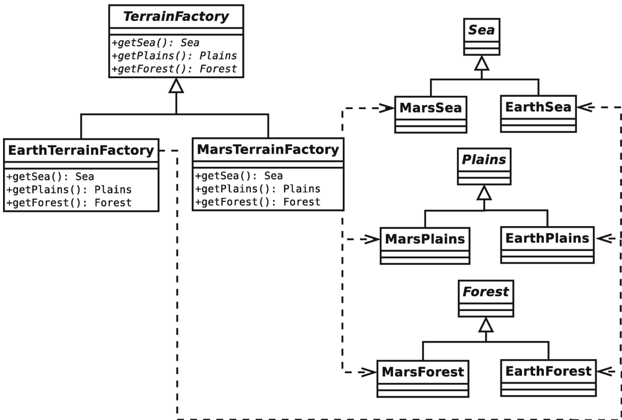
Figure 9-10 Handling terrains with the Abstract Factory method
