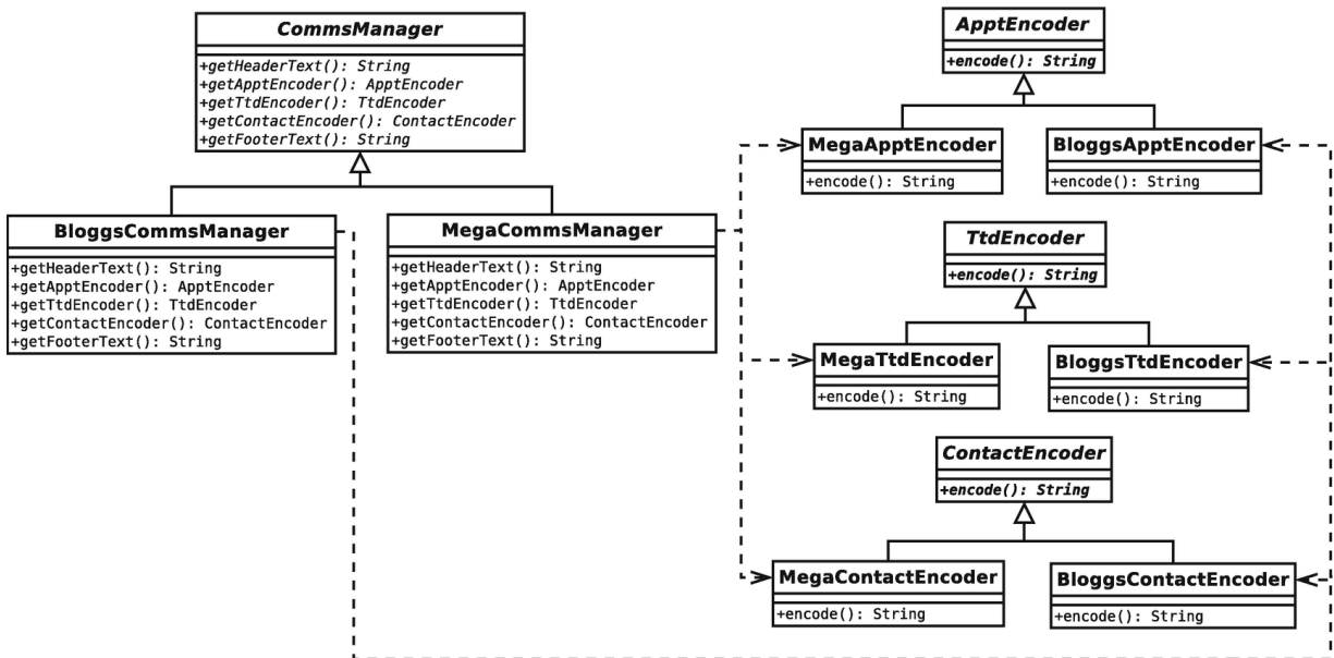
Figure 9-9 Adding concrete creators and some concrete products
