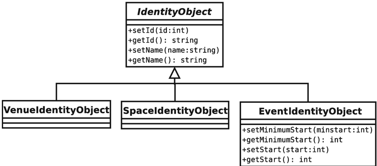
Figure 13-8 Managing query criteria with identity objects
