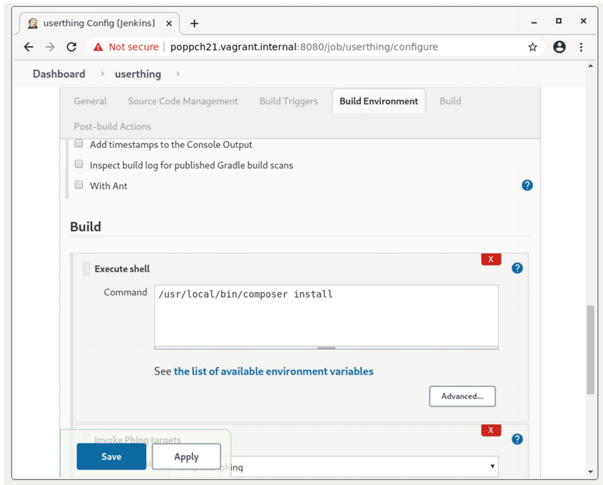
Figure 21-7 Setting up shell execution
