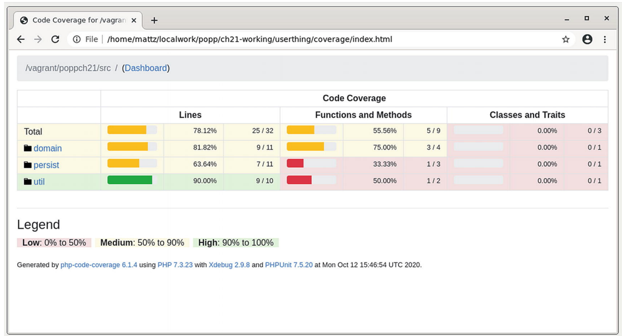
Figure 21-1 The code coverage report
