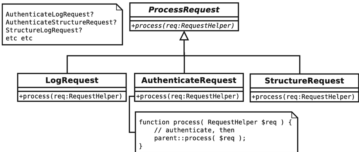
Figure 10-4 More hard-coded variations
