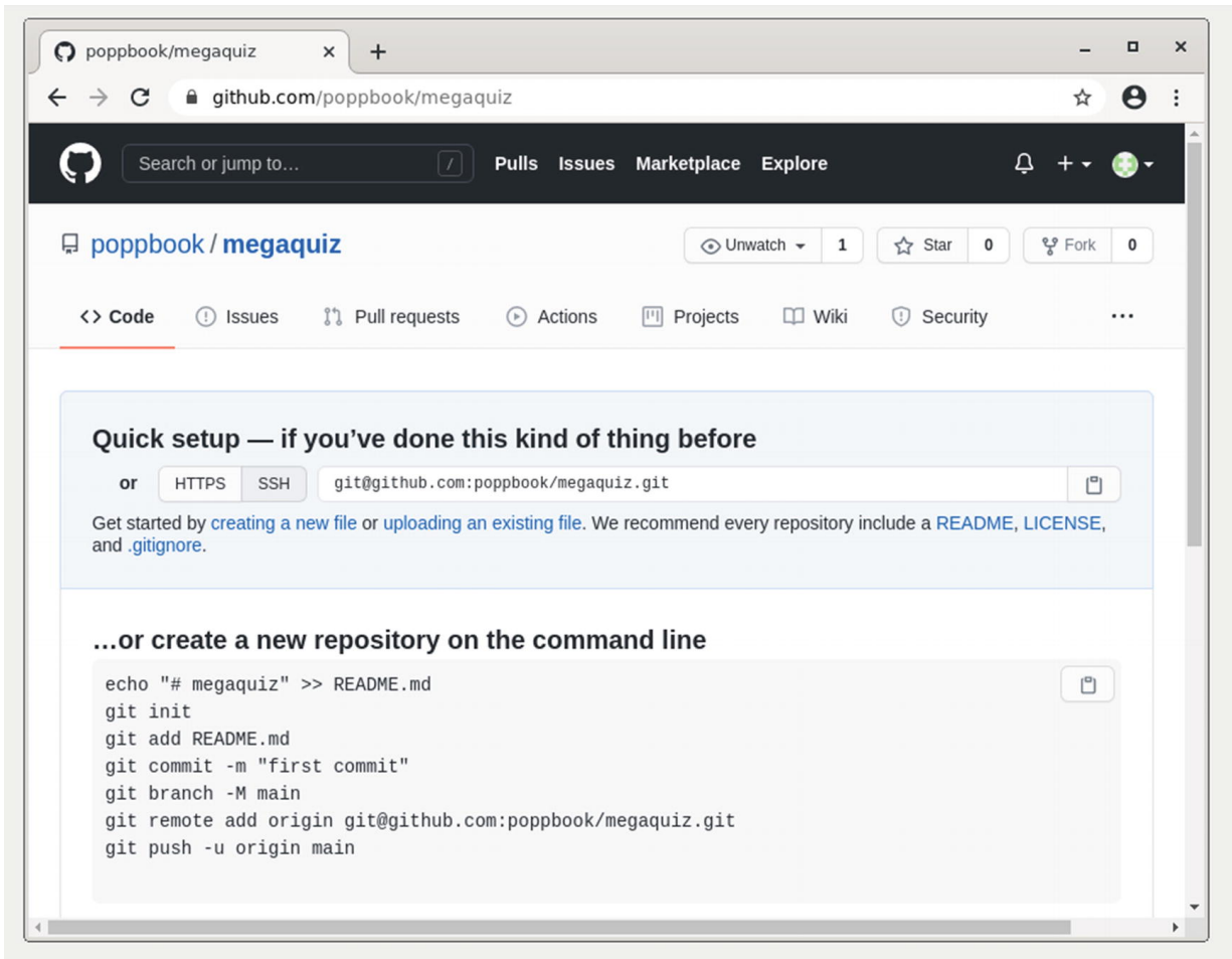
Figure 17-2 GitHub's import instructions
