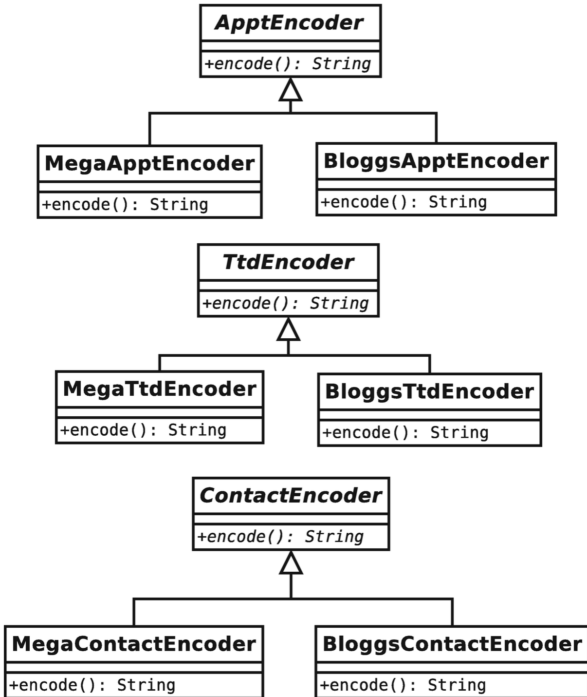
Figure 9-6 Three product families
