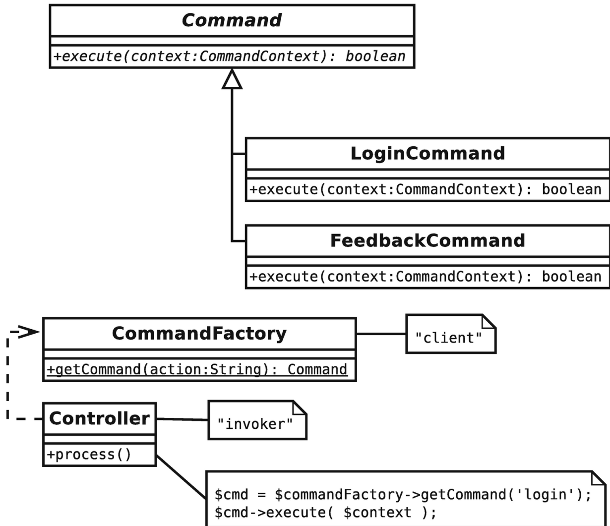
Figure 11-9 Command pattern participants
