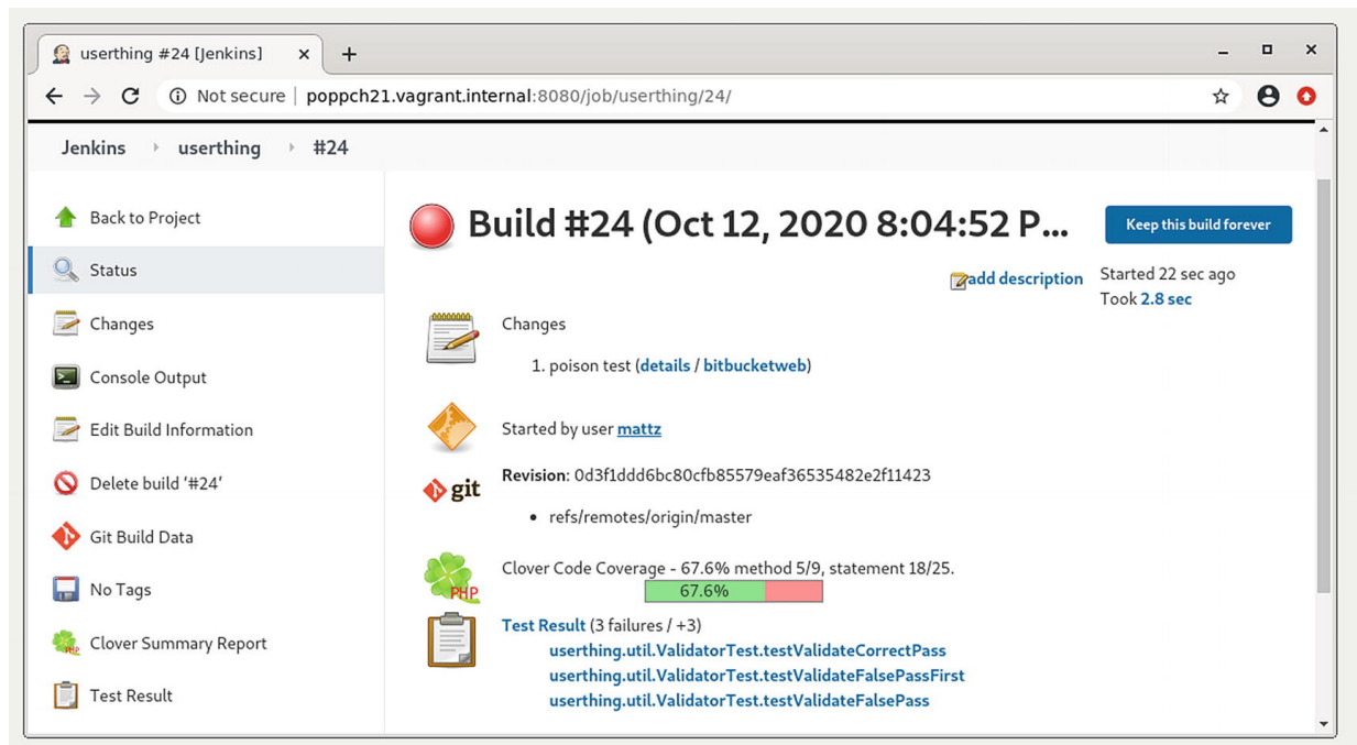
Figure 21-14 The failing build
