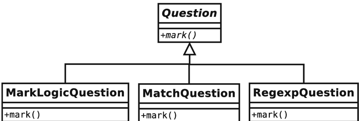
Figure 11-3 Defining subclasses according to marking strategies
