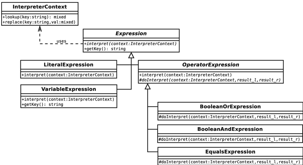
Figure 11-2 The Interpreter pattern deployed
