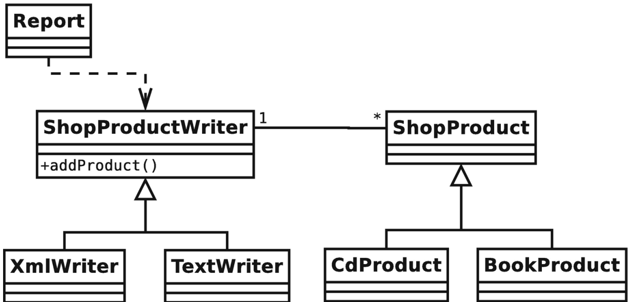
Figure 6-16 A dependency relationship
