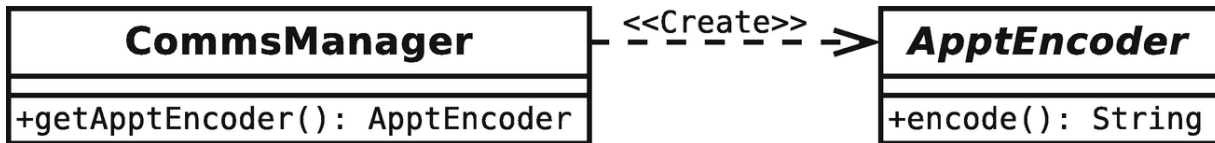
Figure 9-3 Abstract creator and product classes
