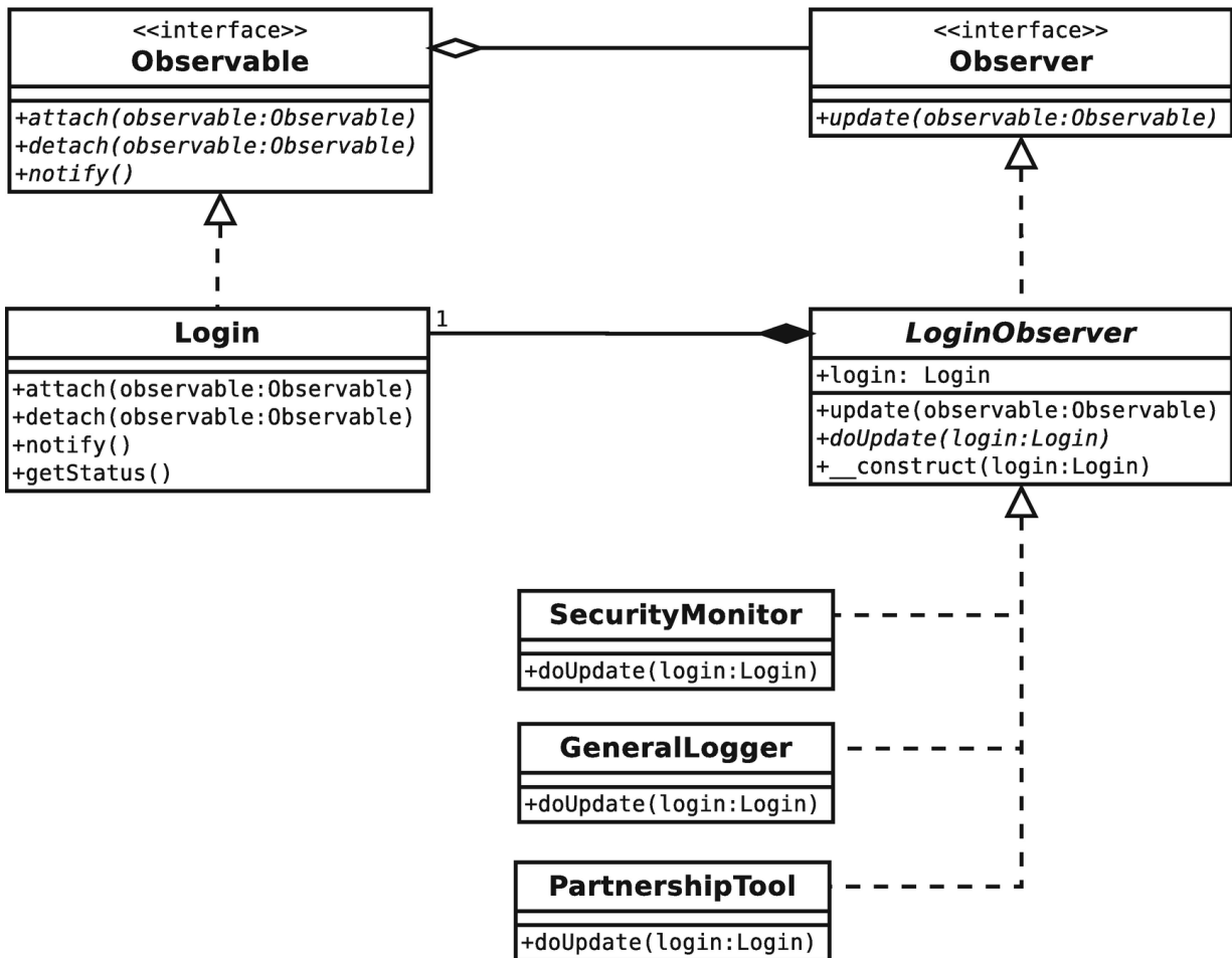
Figure 11-6 The Observer pattern
