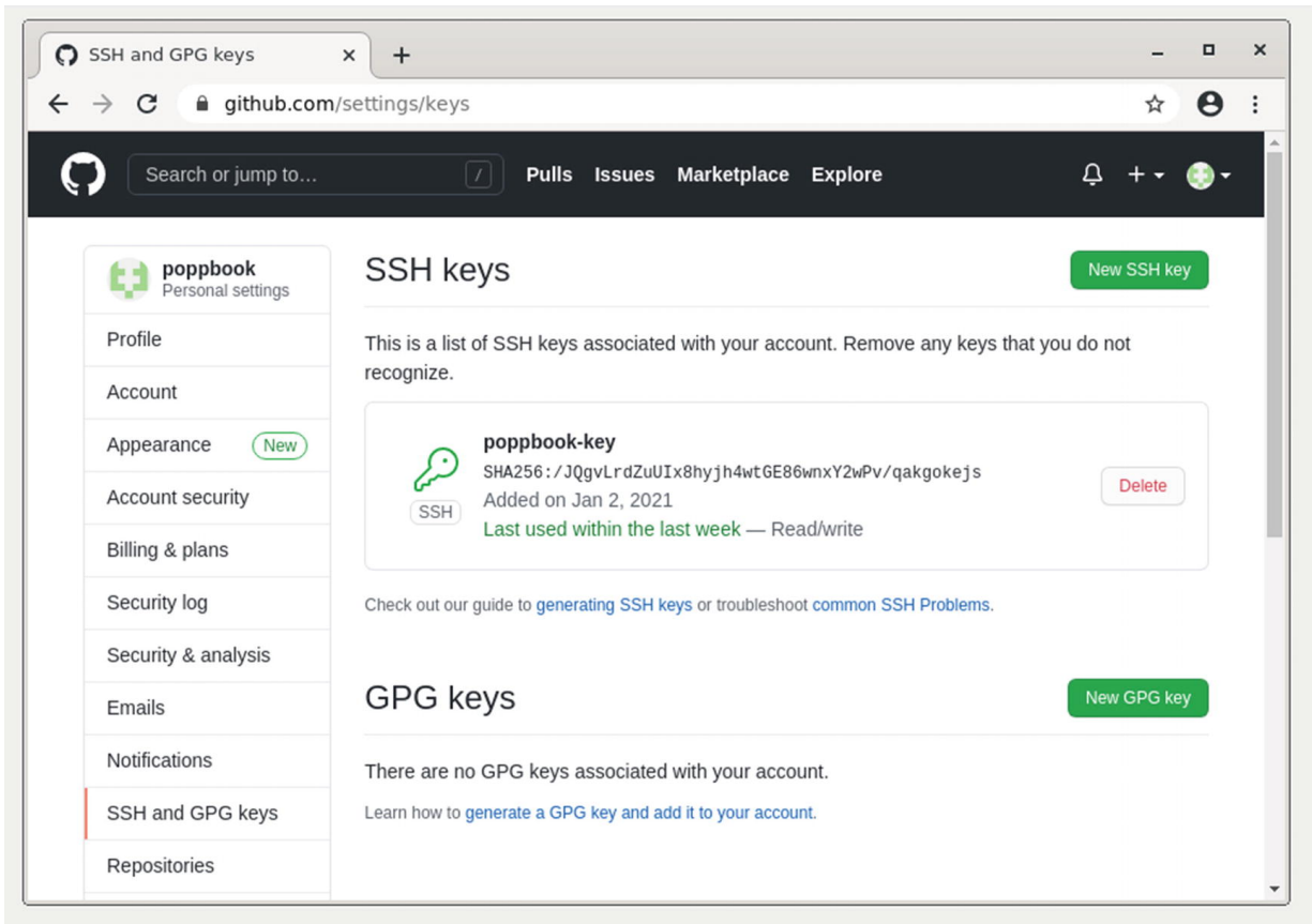
Figure 17-3 Adding an SSH key
