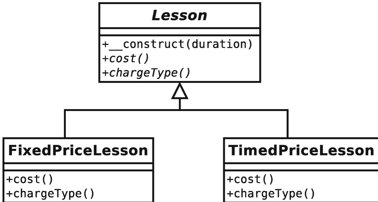
Figure 8-1 A parent class and two child classes
