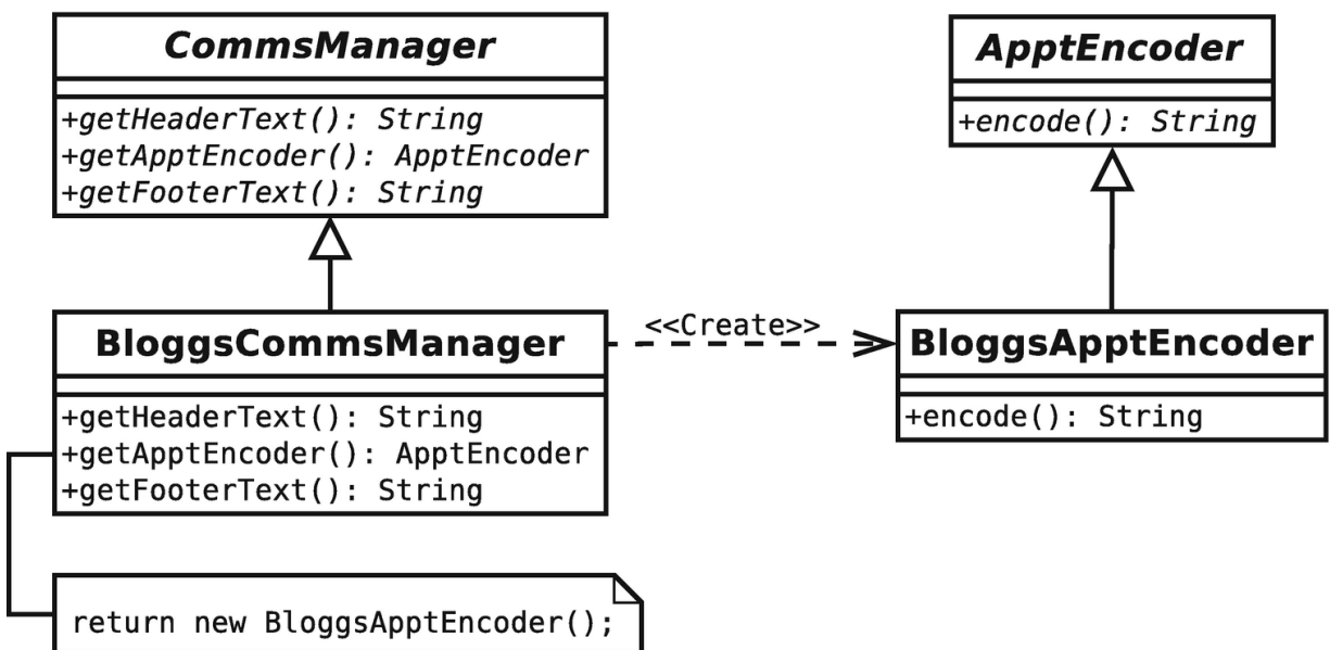
Figure 9-4 Concrete creator and product classes
