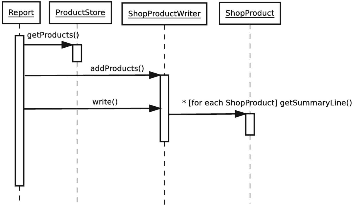
Figure 6-20 The complete sequence diagram
