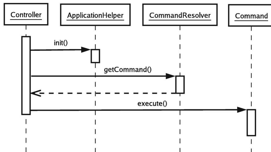
Figure 12-4 The Front Controller in operation
