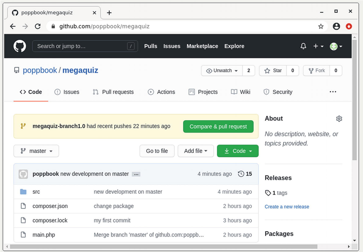
Figure 17-5 GitHub makes issuing pull requests easy
