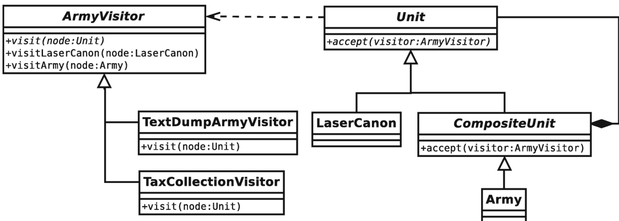
Figure 11-7 The Visitor pattern
