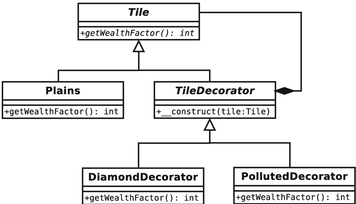
Figure 10-5 The Decorator pattern
