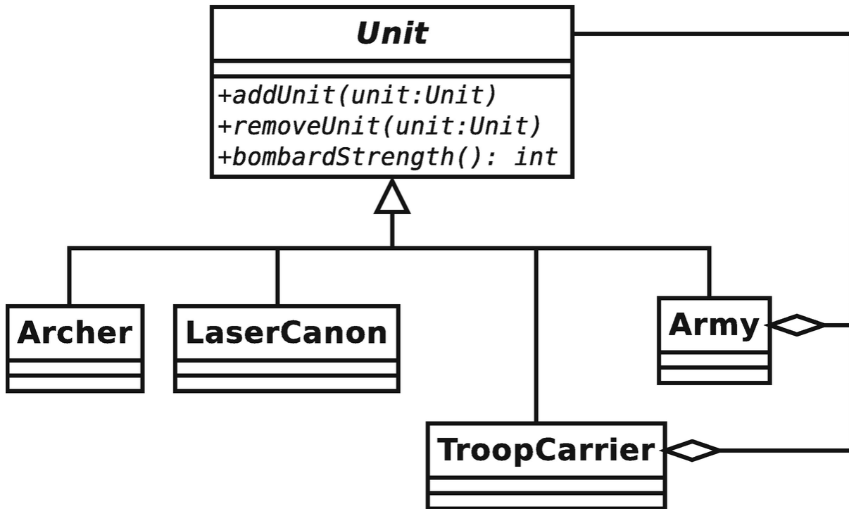
Figure 10-1 The Composite pattern
