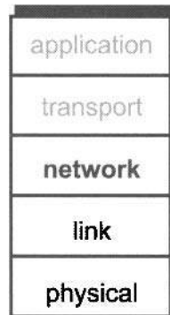
Figure 8.10: Packet Filter
