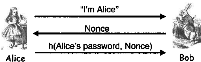
Figure 9.7: Challenge-Response
