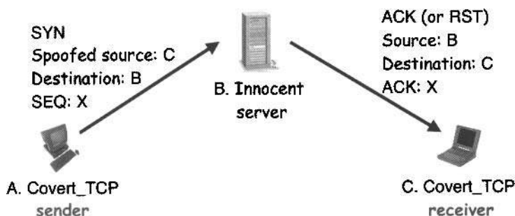
Figure 8.6: Covert Channel Using TCP Sequence Number
