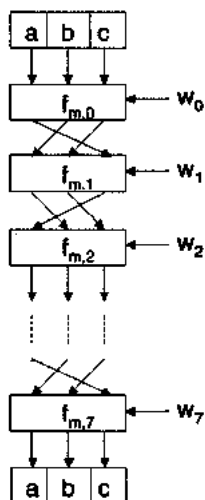
Figure 5.3: Tiger Inner Round for F_m
