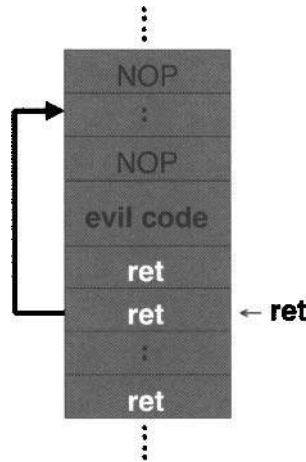
Figure 11.7: Improved Evil Buffer Overflow
