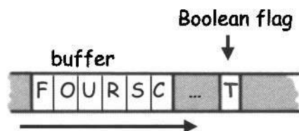
Figure 11.2: Simple Buffer Overflow
