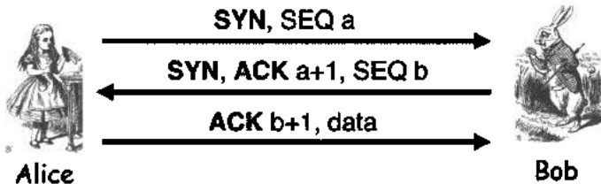
Figure 9.27: TCP 3-Way Handshake
