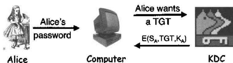
Figure 10.19: Kerberized Login
