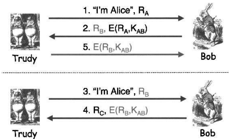
Figure 9.11: Trudy's Attack
