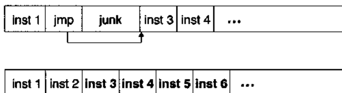
Figure 12.10: False Disassembly
