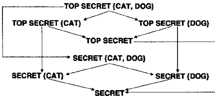
Figure 8.4: Compartments Example
