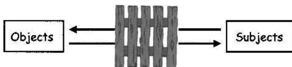
Figure 13.5: Reference Monitor
