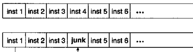
Figure 12.11: Anti-Debugging Example
