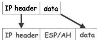
Figure 10.15: IPsec Transport Mode
