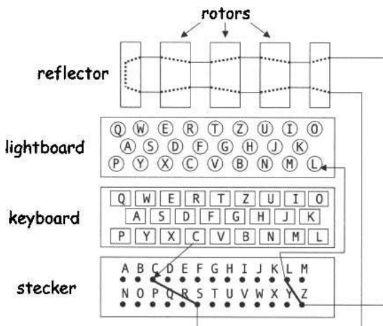
Figure 6.1: Enigma Diagram
