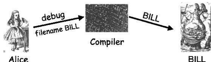
Figure 8.2: Confused Deputy
