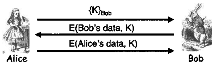
Figure 4.4: Hybrid Cryptosystem
