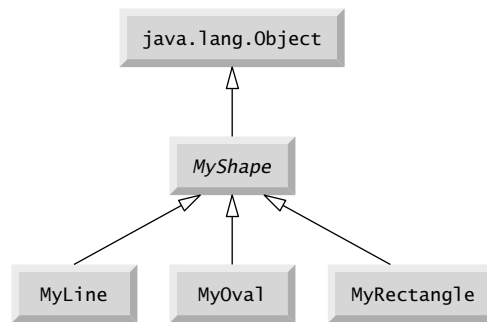
Fig. 10.16 | MyShape hierarchy.
