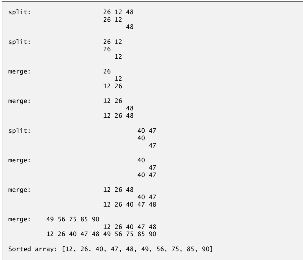
Fig. 19.6 | Sorting an array with merge sort. (Part 4 of 4.)
